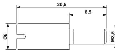
Dimensional drawing
